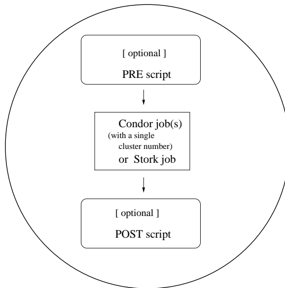
Figure 2.1: One Node within a DAG
